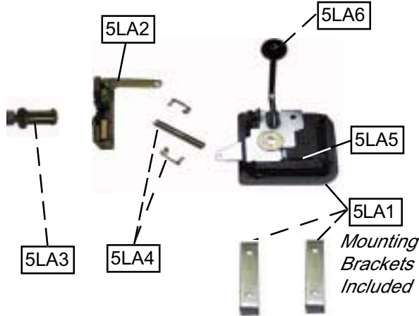
5LA COMPLETE ASSEMBLY
