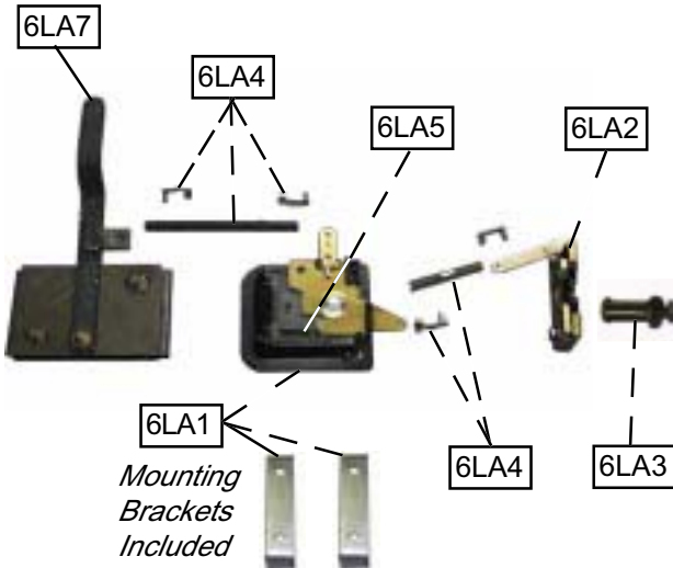
6LA COMPLETE ASSEMBLY
