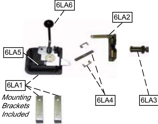
6LA COMPLETE ASSEMBLY
