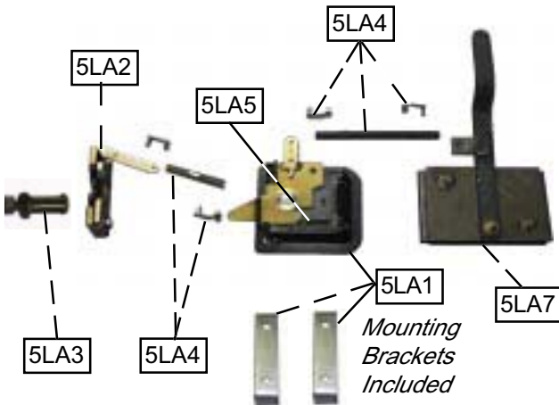
5LA COMPLETE ASSEMBLY
